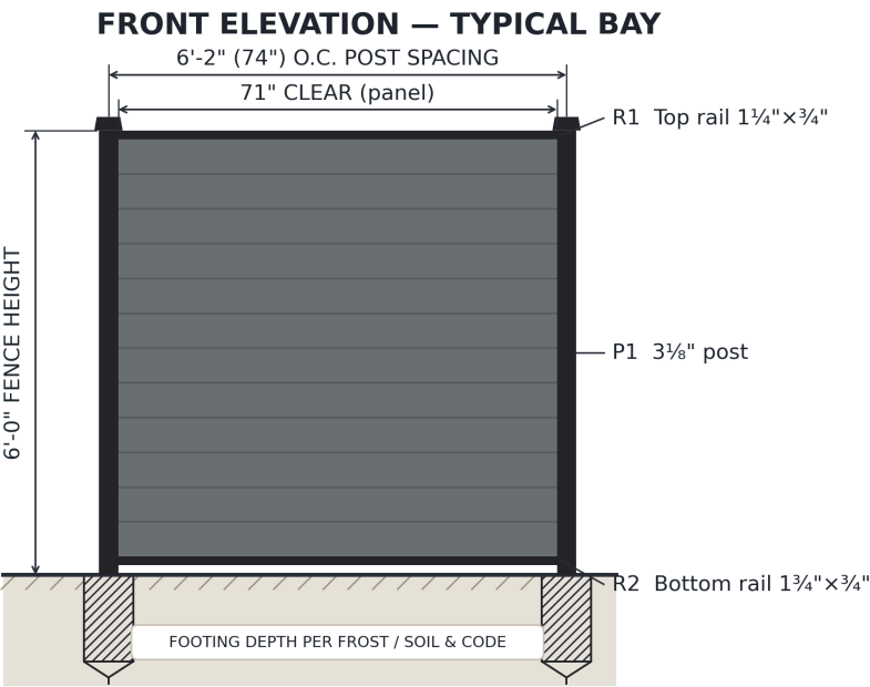
Storm Grey shown · 6 ft x 6 ft full-privacy panel · front elevation, typical bay
